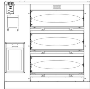
Rear (pass-through)
